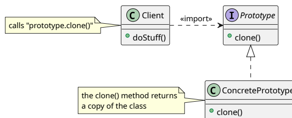
Figure 310: Diagram of the Prototype Pattern
